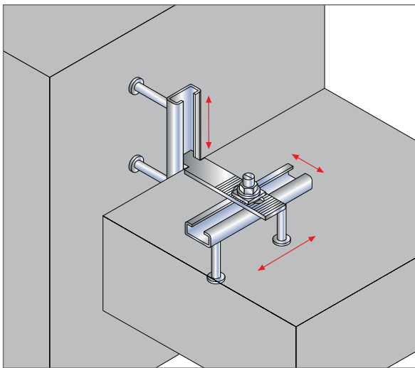
JORDAHL® toothed straps JVB-Z for three-dimensional alignment.
