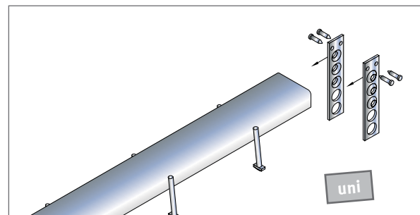
JTB-uni channel with JTB-EB end anchors.
