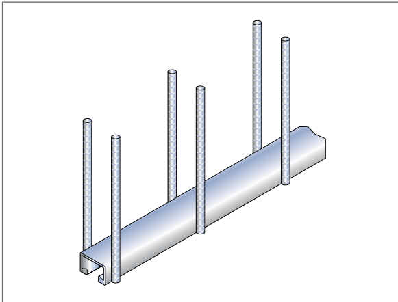
Anchor channel type JRA with reinforcing steel anchors welded on both sides.
