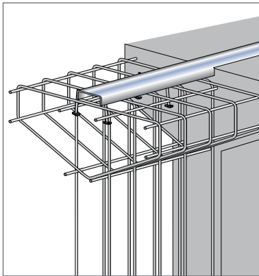
Installation in heavily reinforced elements
