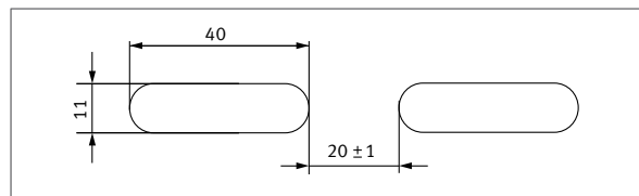
Standard slot pattern 11 x 40
