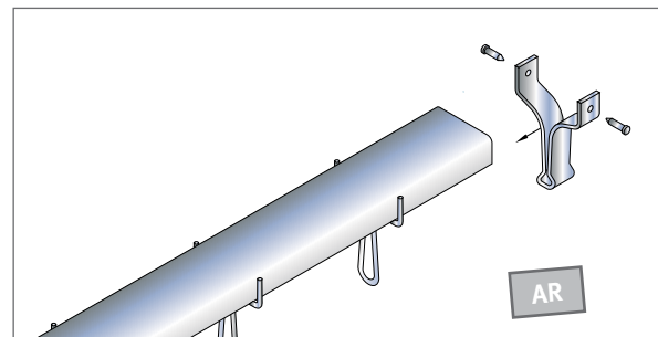
JTB-AR channel with JTB-EA end anchors.
