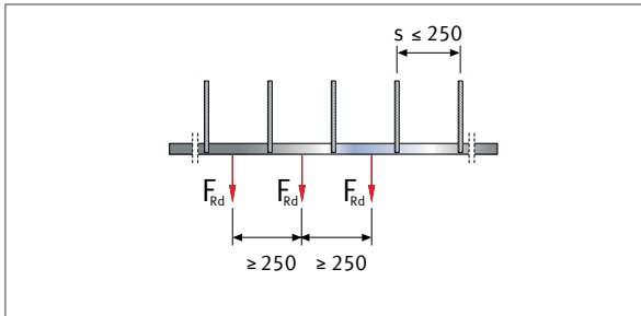
Load arrangement, single load.
