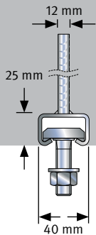
JGB K 40/25 N_{Rd} = V_{Rd} = 11.1 \text{ kN}
