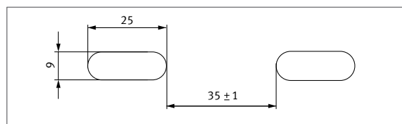
Standard slot pattern 9 x 25
