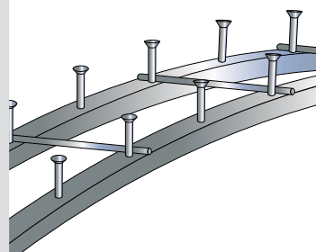
JORDAHL® Curved Anchor Channels
