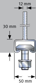
JGB K 50/30 N_{Rd} = V_{Rd} = 17.2 \text{ kN}
