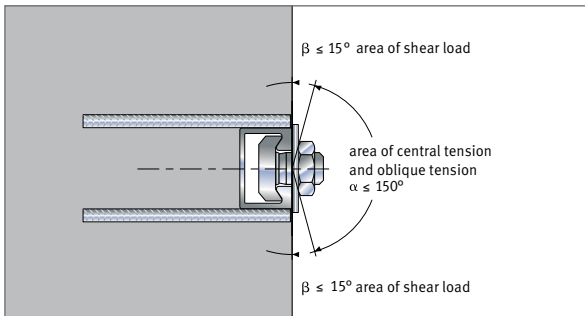
Load ranges.
