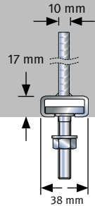
JGB K 38/17 N_{Rd} = V_{Rd} = 10.0 \text{ kN}
