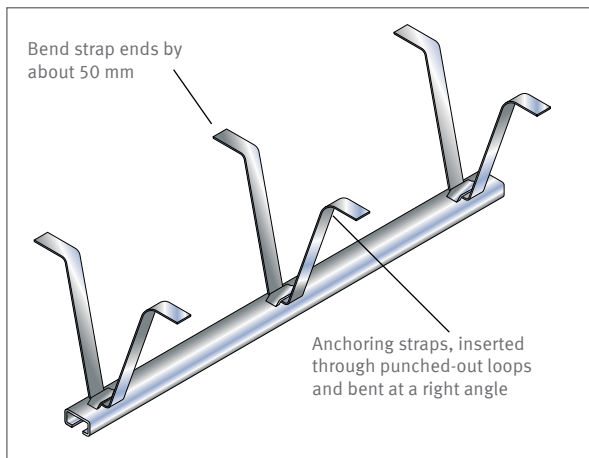
Anchor channel JSA with installed straps.
