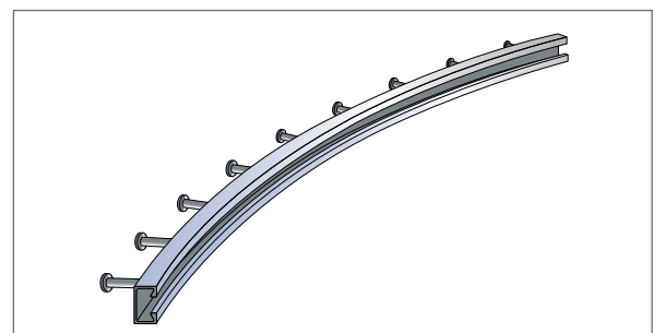
Curved anchor channel for tunnel construction.
