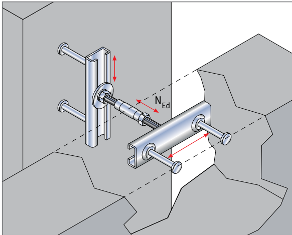
Turnbuckle Connections JSV provide three-dimensional alignment.
