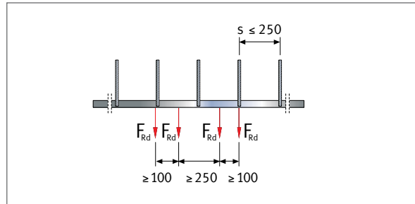
Load arrangement, load pairs.
