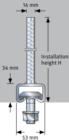
JGB K 53/34 N_{Rd} = V_{Rd} = 30.6 \text{ kN}
