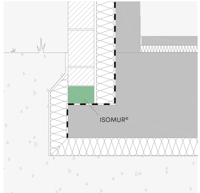
ISOMUR® in non load-bearing exterior wall
